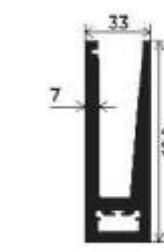
Continuous Railing Bottom Section Number: V-10001 Weight (kg/12'): 15.775
