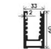
Continuous Railing Bottom Section Number: V-10004 Weight (kg/12'): 6.850
