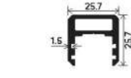
Continuous Railing Top Section Number: V-10056 Weight (kg/12'): 2.150
