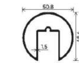
Continuous Railing Top Section Number: V-10051 Weight (kg/12'): 3.200
