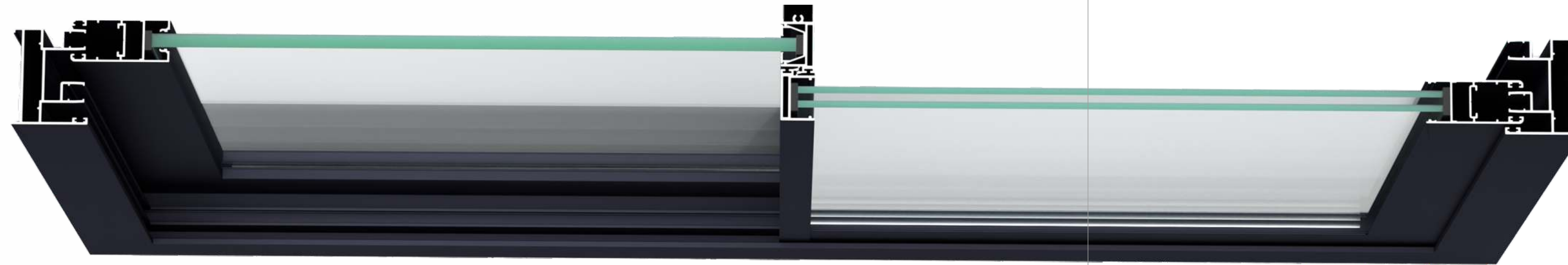
Top View
