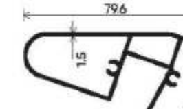
Continuous Railing Top Section Number: V-10055 Weight (kg/12'): 4.100
