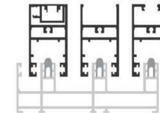
Three Track with Mosquito Assamble
