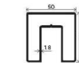
Continuous Railing Top Section Number: V-10053 Weight (kg/12'): 4.600
