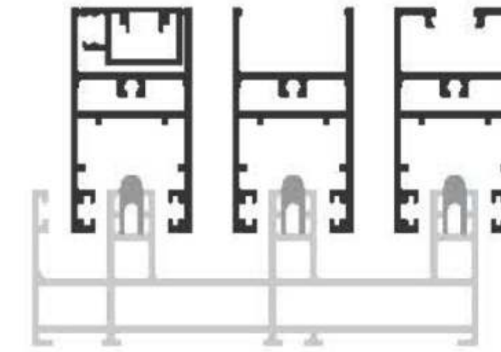
Three Track with Mosquito Assemble
