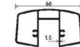
Continuous Railing Top Section Number: V-10054 Weight (kg/12'): 4.080
