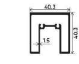
Continuous Railing Top Section Number: V-10052 Weight (kg/12'): 3.400
